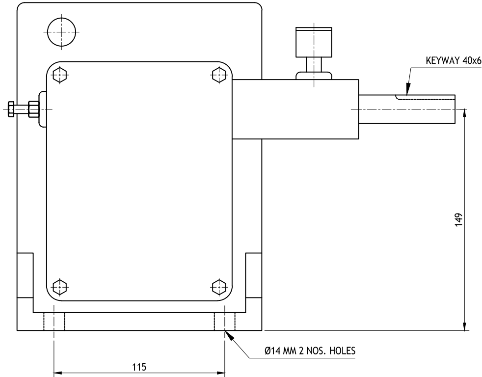
ROTARY GEARED LIMIT SWITCH (IP - 44)
